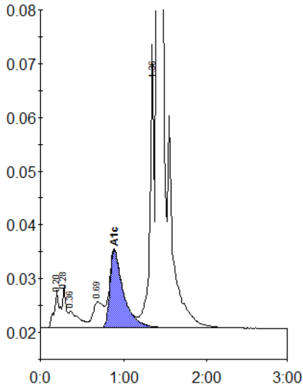
Peak table - ID: 10611340
